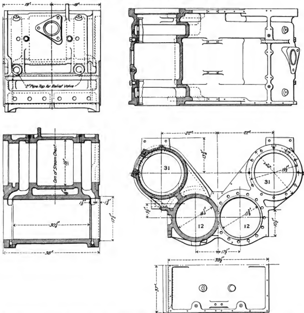
Figs. 810-844. High Pressure Cylinders and Steam Chests of Cole Four-Cylinder Balanced Compound Locomotive, Diameter 16 \frac{1}{4} in. American Locomotive Co.
